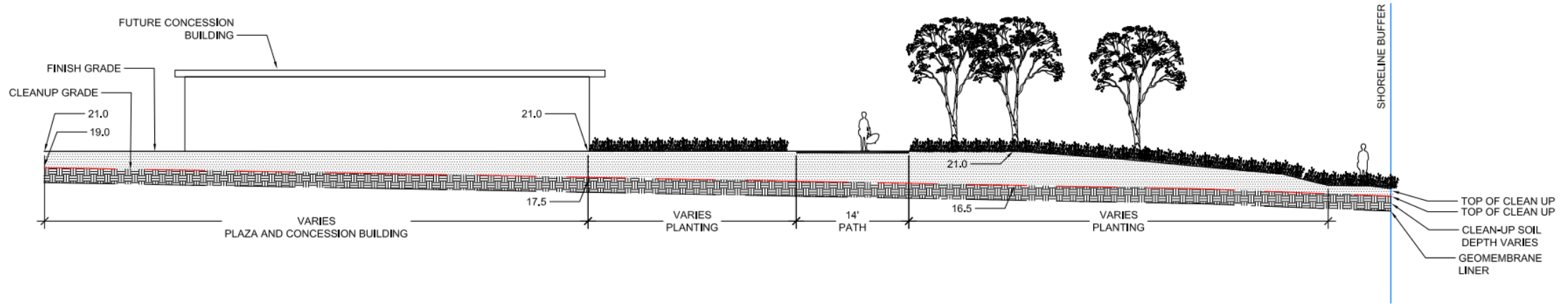
1 SECTION AT FUTURE PLAZA AND CONCESSION BUILDING AT RG HALEY
