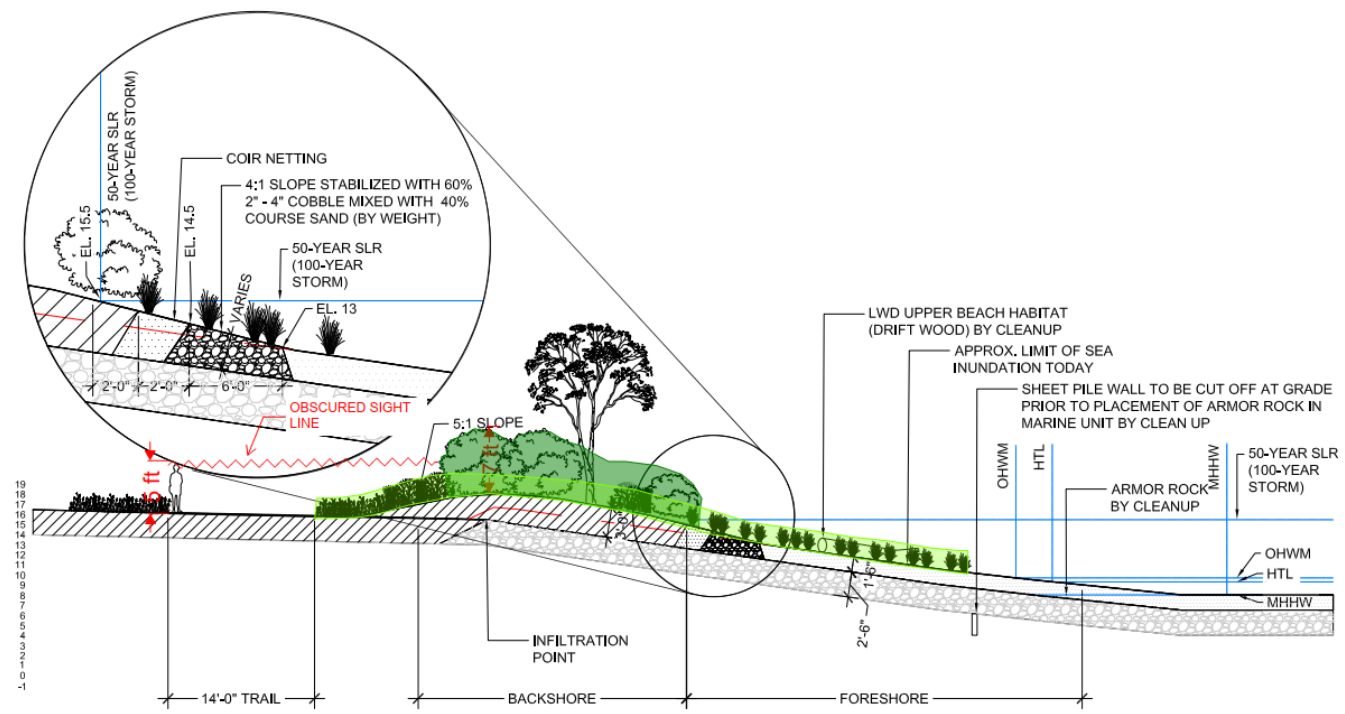
1 RG HALEY BACKSHORE MITIGATION SECTION WITH ADDED SOIL VOLUME SCALE: 1/8" = 1'-0"
