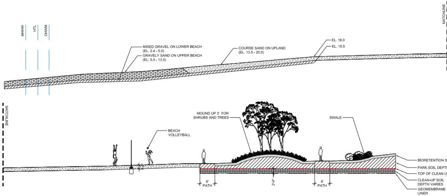
1 SECTION AT SOUTH BEACH SCALE: 1/8" = 1'-0"
