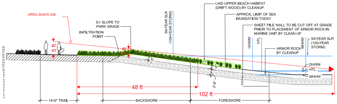
1 RG HALEY BACKSHORE MITIGATION SECTION WITH ADDED SOIL VOLUME SCALE: 1/8" = 1'-0"
